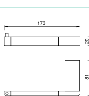
TOILET ROLL HOLDER (7)644945
