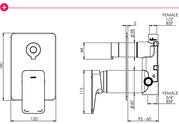
SHOWER MIXER DIVERTER (7)686615
