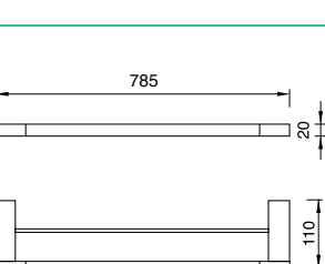
TOWEL RAIL DOUBLE 750 (7)644944
