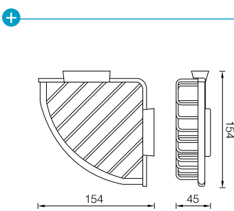
TRIANGULAR SOAP BASKET SMALL (7)645841
