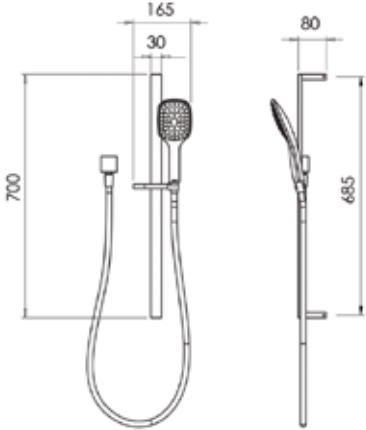
SLIDE SHOWER (7)711718 WELs Rating 2 ★
