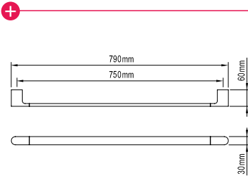
TOWEL RAIL SINGLE (7)620992
