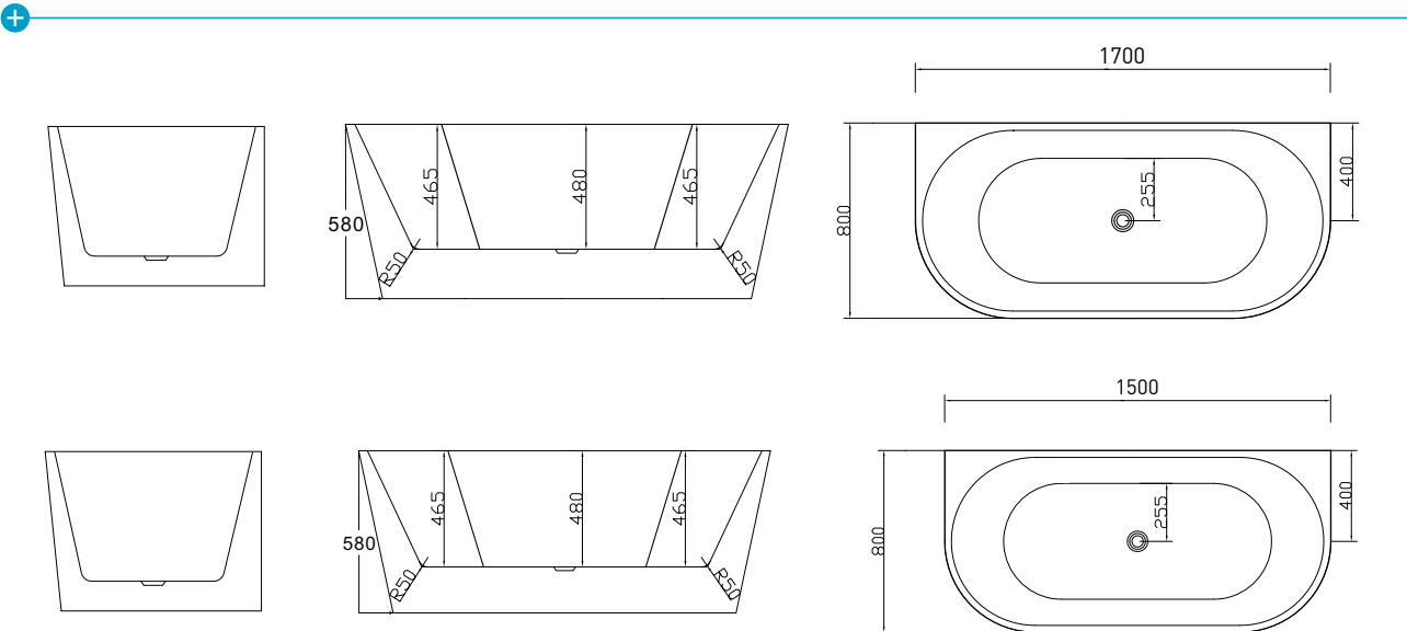
SOL FREESTANDING BATH (7)711719 / (7)749990
