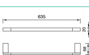
TOWEL RAIL SINGLE 600 (7)644940
