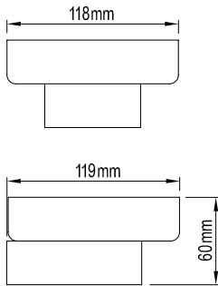
SOAP DISH (7)620988
