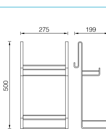
DOUBLE RECTANGULAR RACK (7)645844
