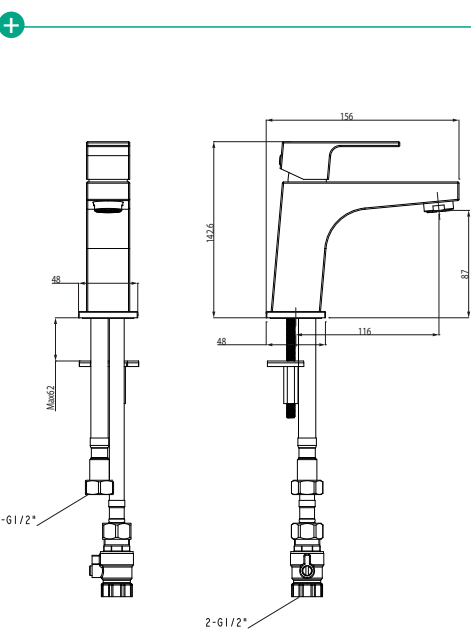
BASIN MIXER (7)686618 WELs Rating 5 ★
