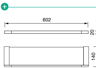
GLASS SHOWER SHELF (7)644951
