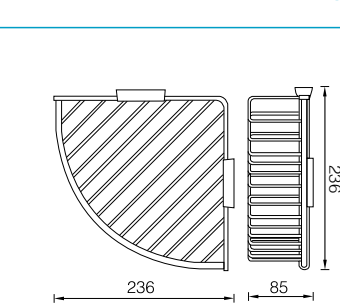
TRIANGULAR SOAP BASKET LARGE (7)645840
