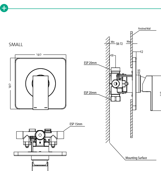
SHOWER MIXER (7)686619
