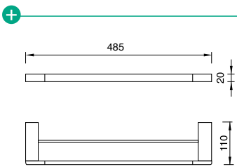
TOWEL RAIL DOUBLE 450 (7)644942
