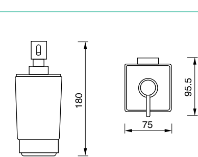
SOAP DISPENSER (7)644950
