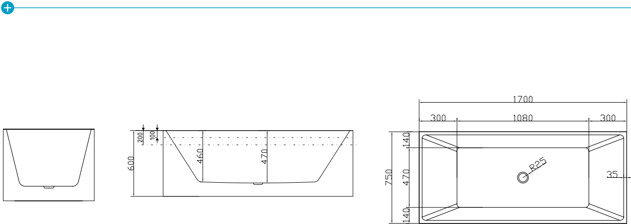
DEGREE FREESTANDING BATH (7)711725
