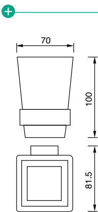
TUMBLER HOLDER (7)644947
