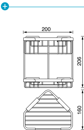
DOUBLE TRIANGULAR SOAP BASKET (7)645843
