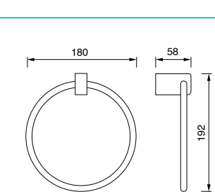
TOWEL RING (7)644949
