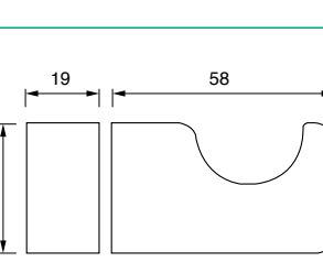
ROBE HOOK (7)644946
