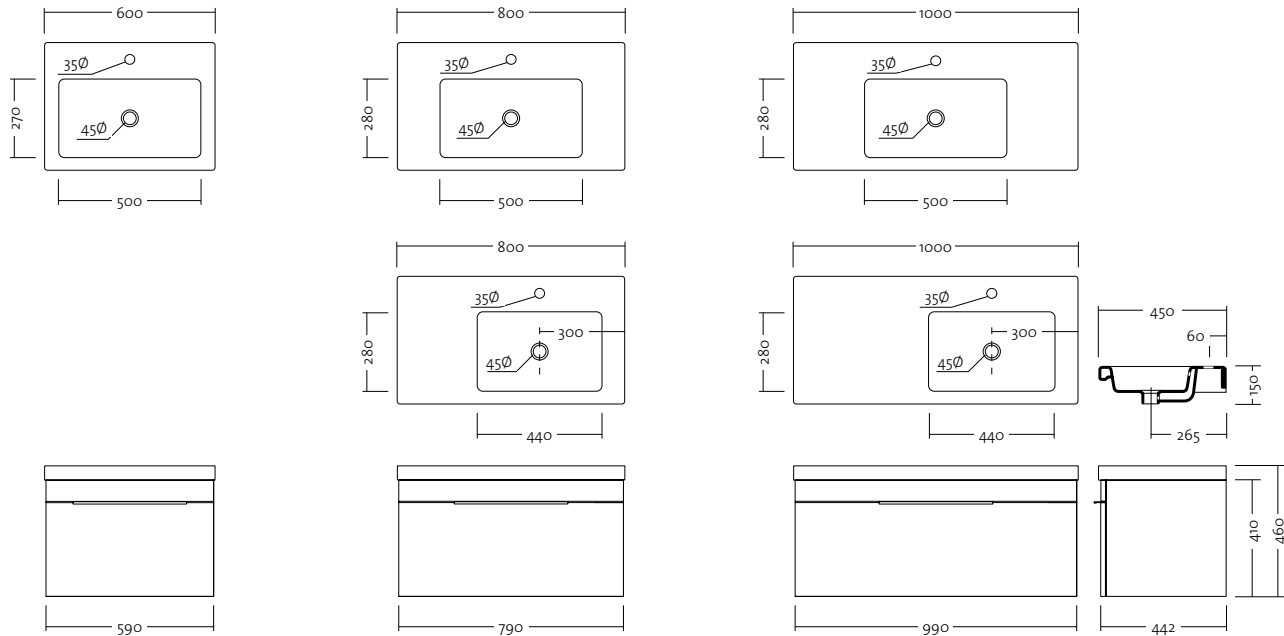
600W x 450D x 460H CENTRE BASIN
