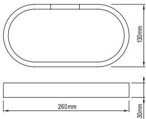
SOAP DISH (7)620988
