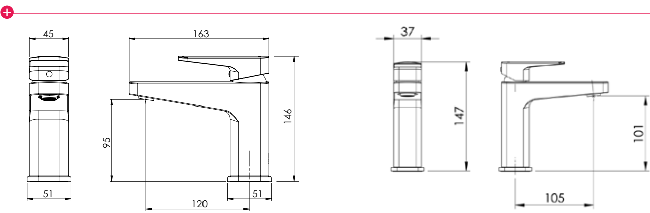
BASIN MIXER (7)686610 WELs Rating 4 ★
