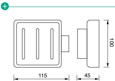
SOAP HOLDER (7)644948
