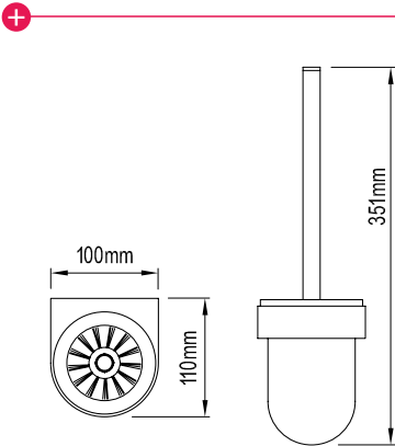
TOILET BRUSH HOLDER (7)620995
