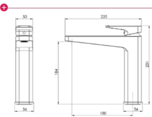
SINK MIXER (7)711717 WELs Rating 4 ★
