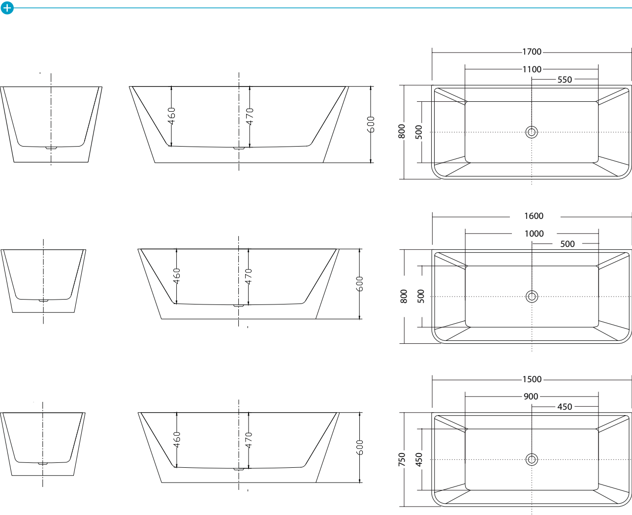
FORM FREESTANDING BATH (7)711720 / (7)749991 / (7)749992
