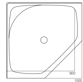
Corner Shower 900 / 1000
