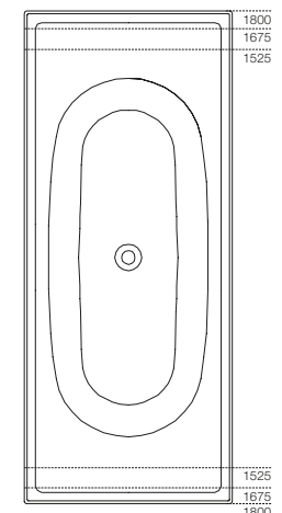
Bath 1800 / 1675 / 1525
