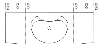
Basin 600 / 900 / 1200
